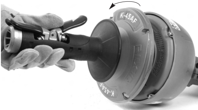
Figure 14 – Twist Drum Apart
